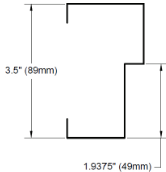
DRAWING PROFILE FOR SINGLE RABBET FRAME DEPTH 3.5"
