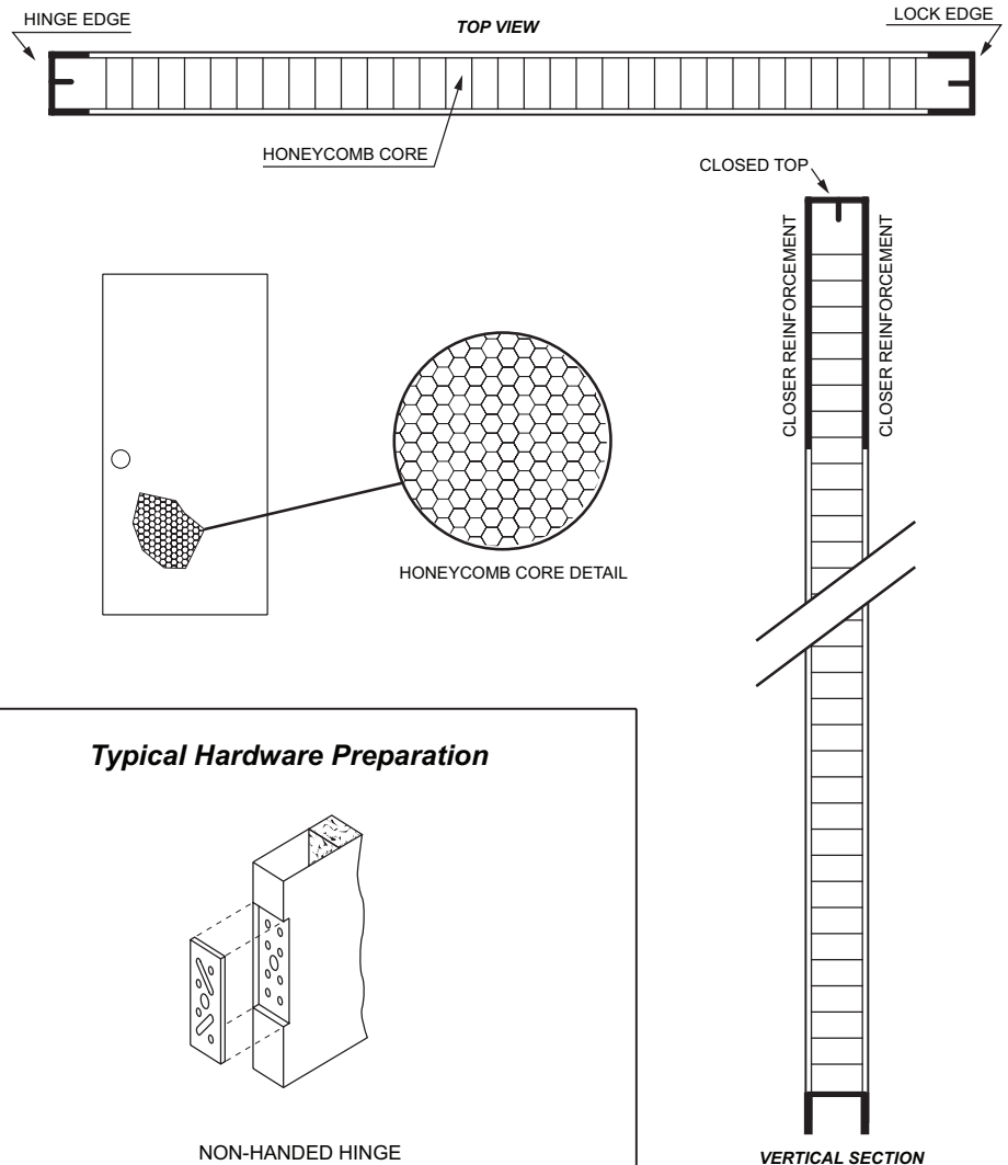
VERTICAL SECTION
