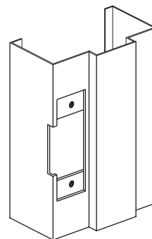
4-7/8" UNIVERSAL STRIKE
