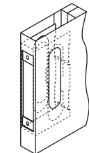
ANSI / SDI A115.1 "MB" (MORTISE)
