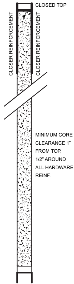
TYPICAL SECTION
