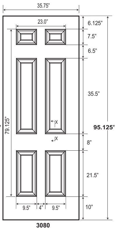
ANSI / SDI A115.2 "C" (BORED)
