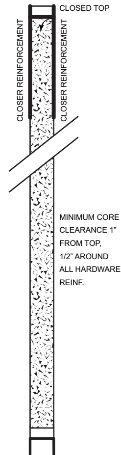
TYPICAL SECTION
